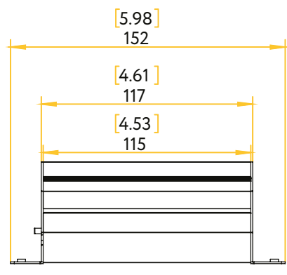
Driver Box for G-96024
